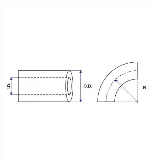
O.D. outside diameter | I.D. inside diameter | R minimum bend radius to the centreline. Nominal, in inches.
