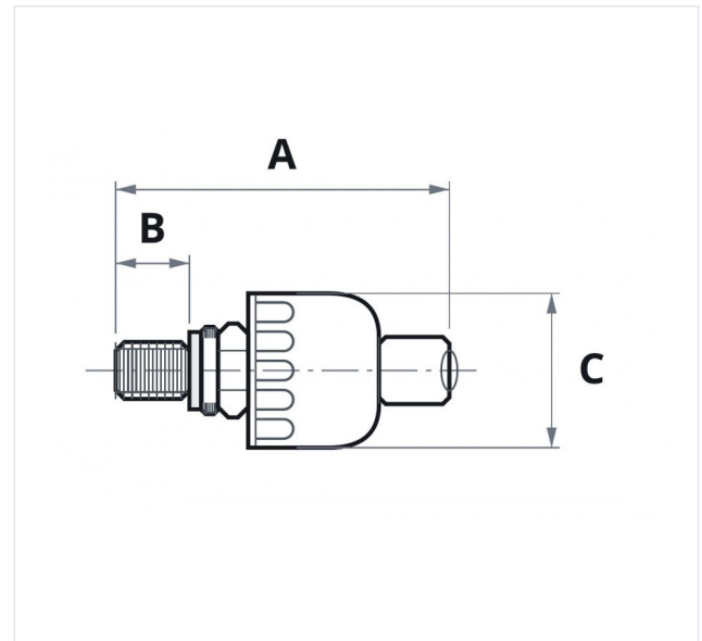
A overall length (height on the 90° sweep) | B thread length | C body diameter (reach on the 90° sweep). Nominal, in inches.
