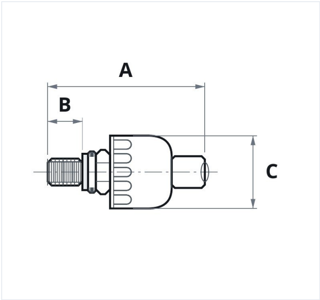
A overall length | B thread length | C body diameter. Nominal, in inches.
